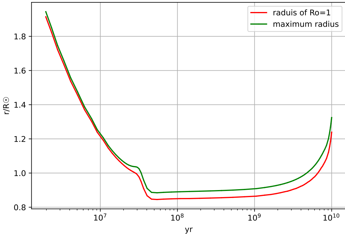
age against radius of Ro=1
